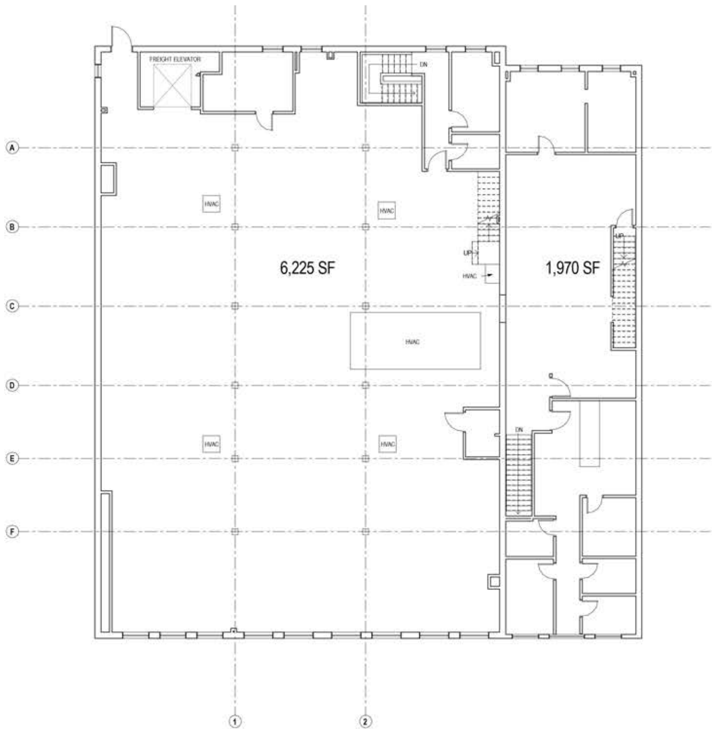
1 SECOND FLOOR 1/8" = 1'-0"
