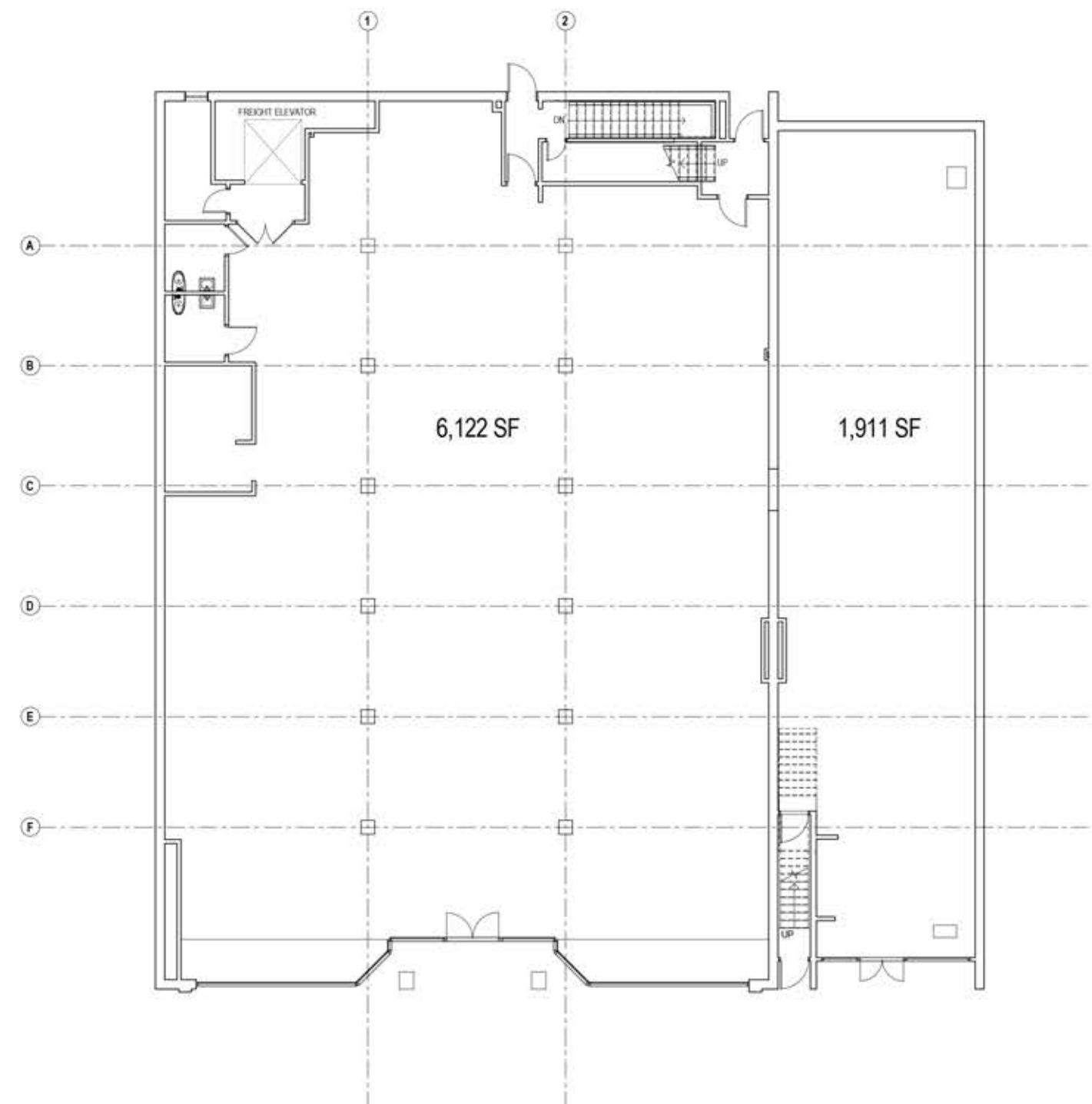
1 FIRST FLOOR 1/8" = 1'-0"
